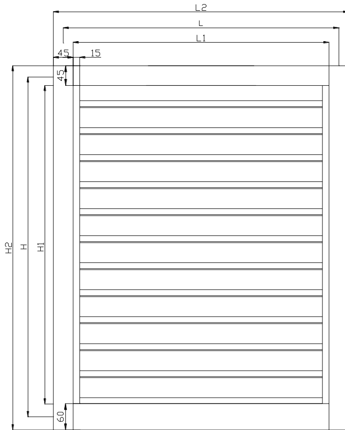
FA-450 – ΟΨΗ (L x H)
