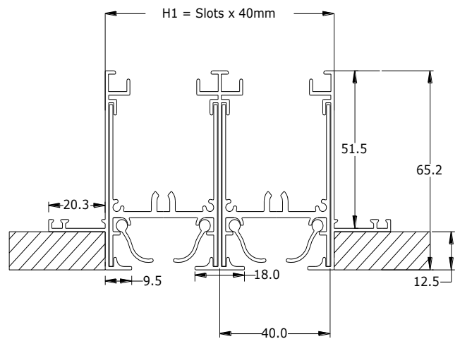
SL-852-P – SECTION
