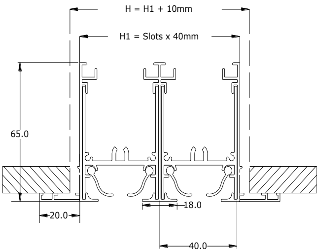
SL-802-P – SECTION
