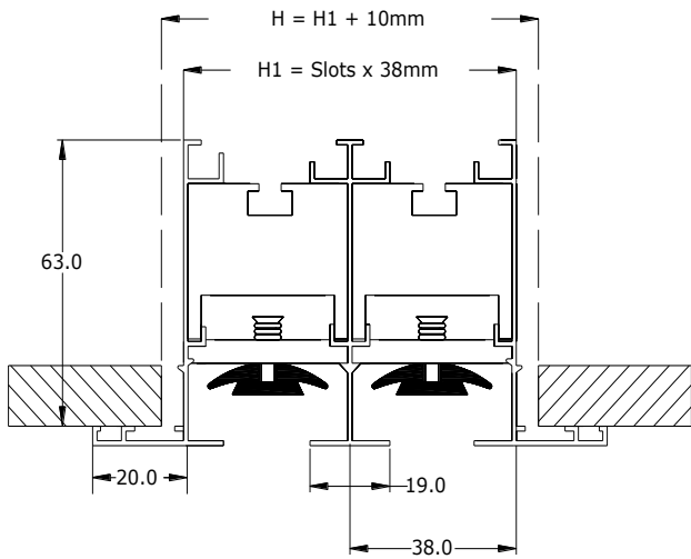
SL-802 – SECTION
