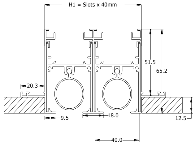
SL-852-S – SECTION
