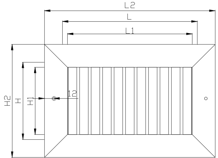
RD-301/302 - VIEW (H x L)
