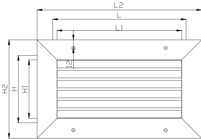
RD-301/302 - VIEW (L x H)
