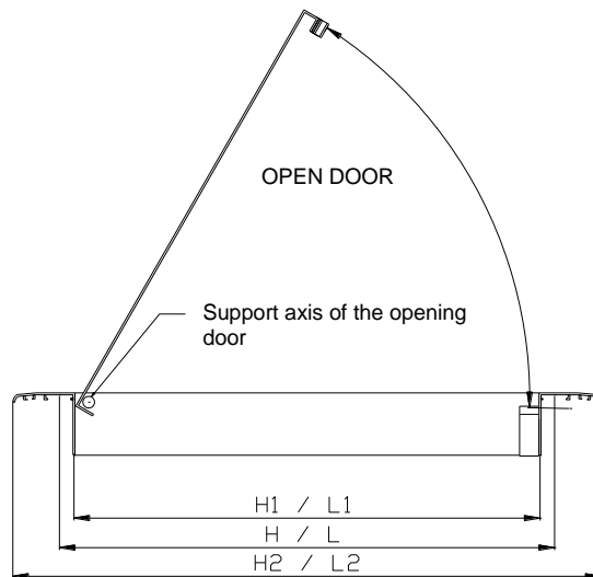
ACDR – SECTION (DOOR OPEN)
