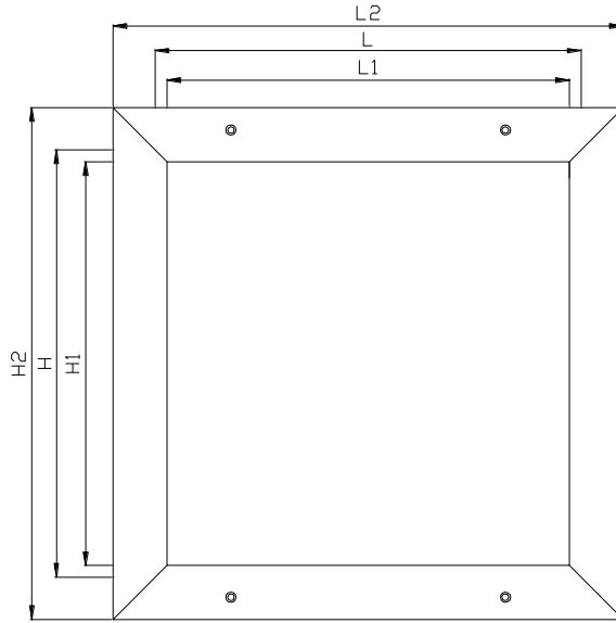
ACDR/CG – VIEW
